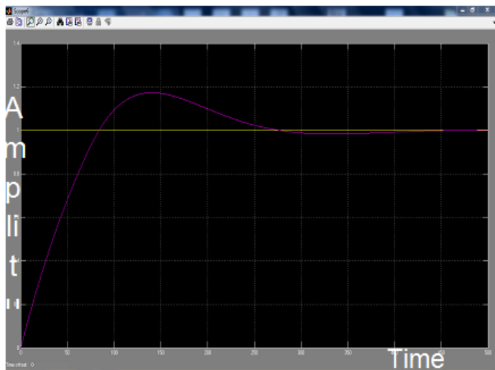
Fig 6: Scope of the unit step response of the system for test 2
