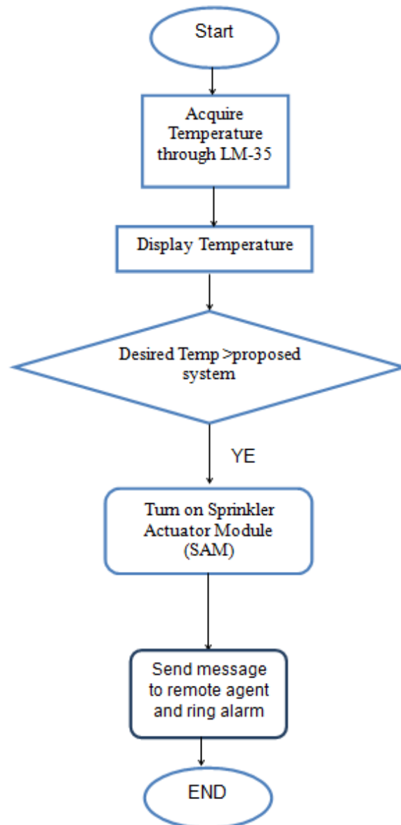
Fig 2: Flow chart for control in a single channel
