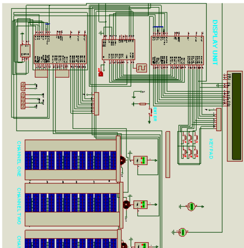
Fig 8: Snapshot capture of the system on Proteus 7.8 after initialization
