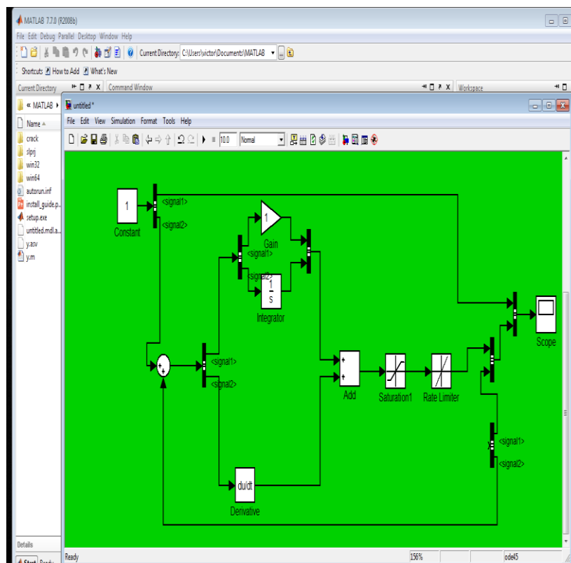
Figure 4: Simulink block diagram of proposed system.
