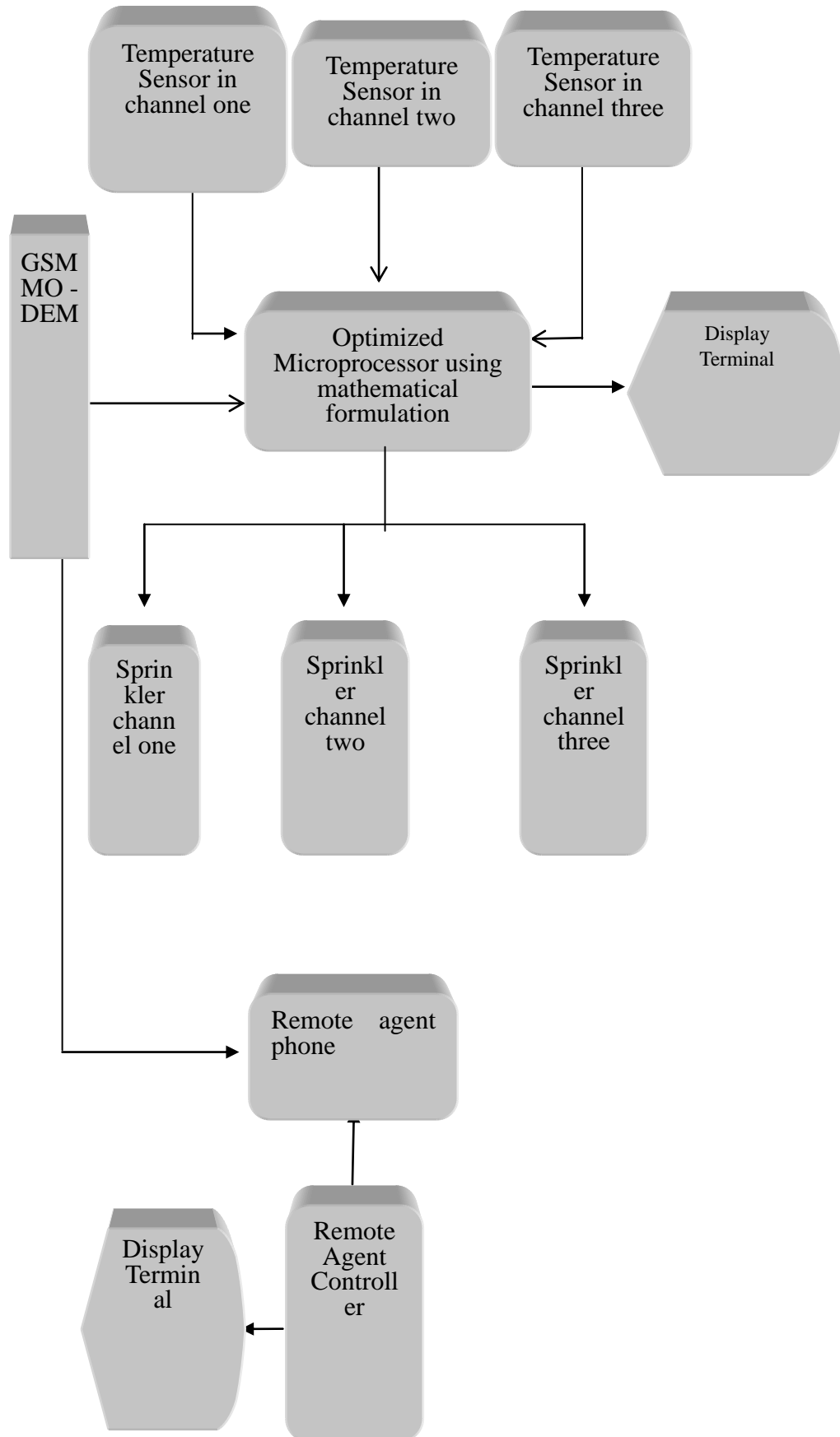
Fig 3: Block diagram of the proposed system showing the flow of information from rooms under observation to Remote Agent Centre.
