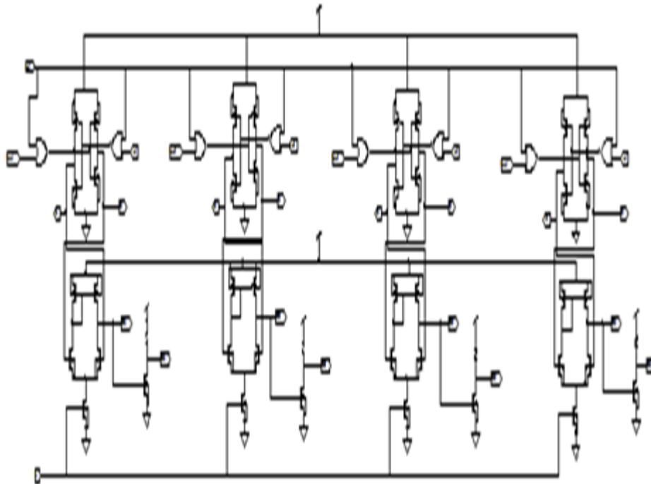
Figure 8: Four bit non-volatile SRAM.
