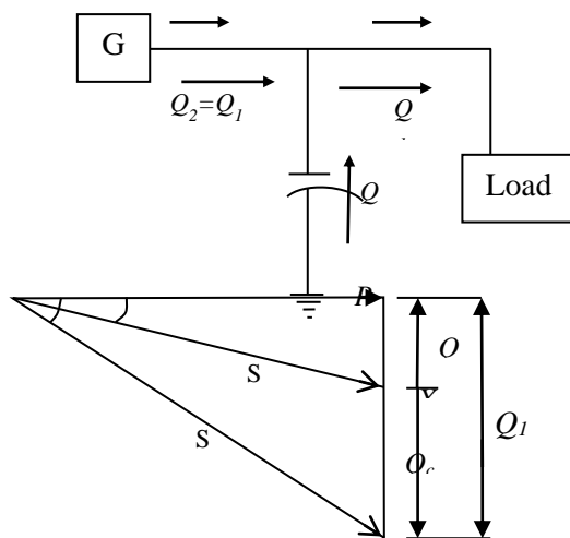
Figure 2: Pythagoras theorem for capacitor compensation (capacitor bank)
