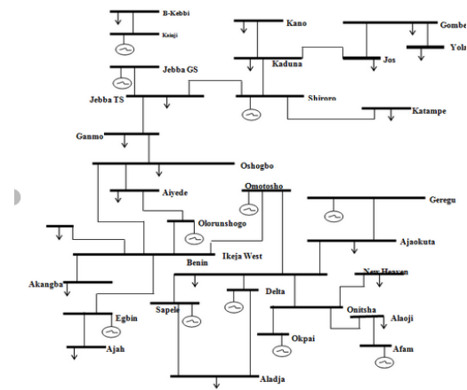
Figure 1: Single line Diagram of 28-Bus, 330kV Nigeria Network.
