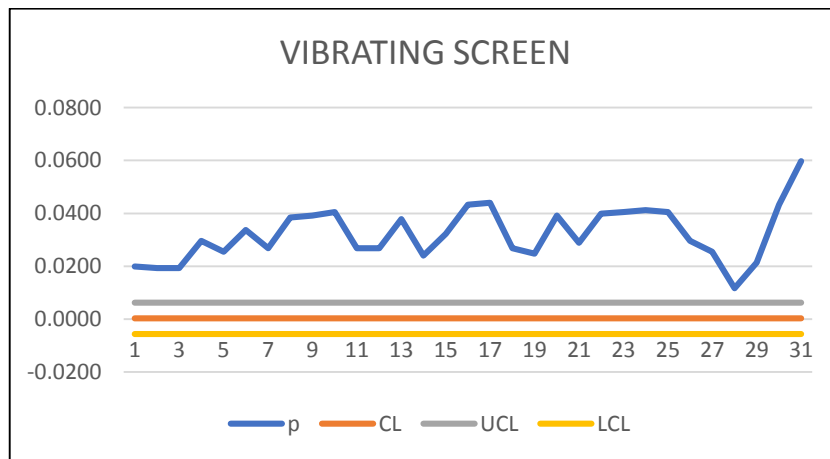
Diagram 4. Full Map p Vibrating Screen
