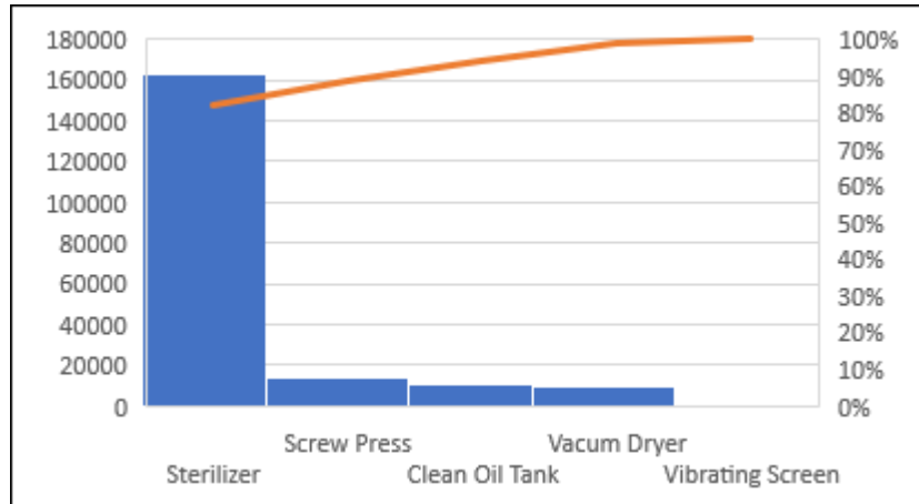
Diagram 5. Production Process Pareto Diagram
