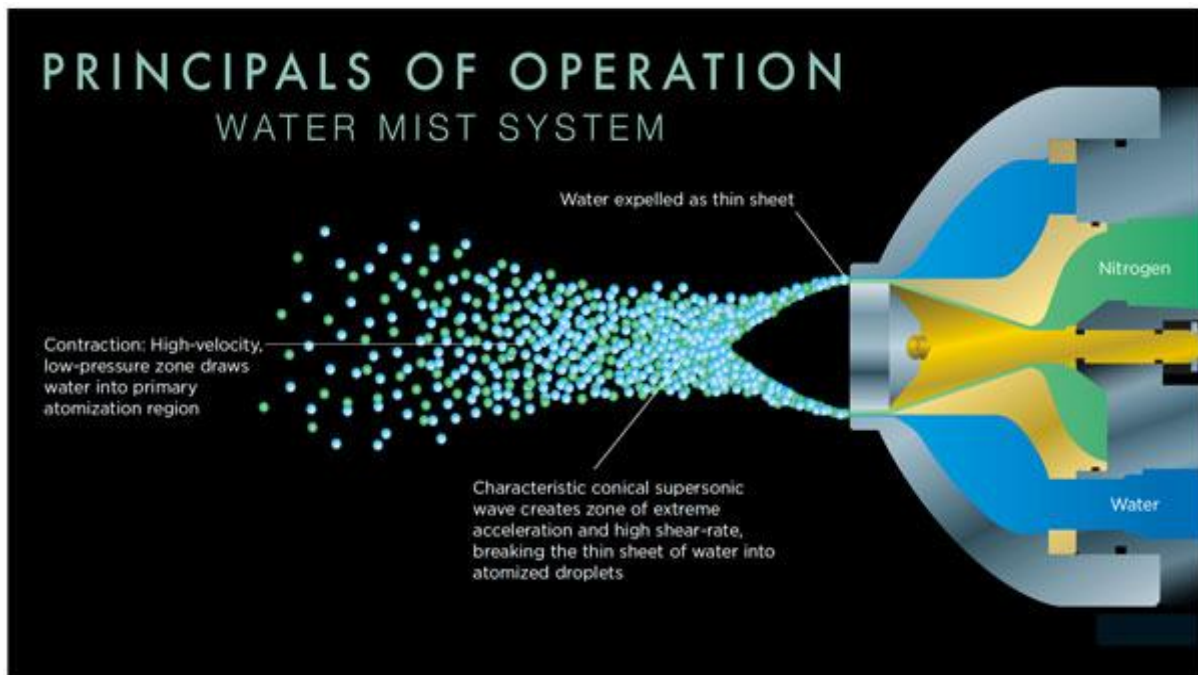
Figure 4: Water mist systems sprays thin water showers or jets in which 99% of the quantity of these sprays formed of drops whose diameter is less than 1000 microns.
