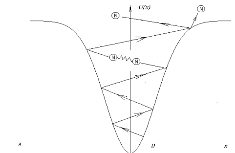
Fig.8. Oscillation of Nitrogen molecule in potential well of catalyst.
