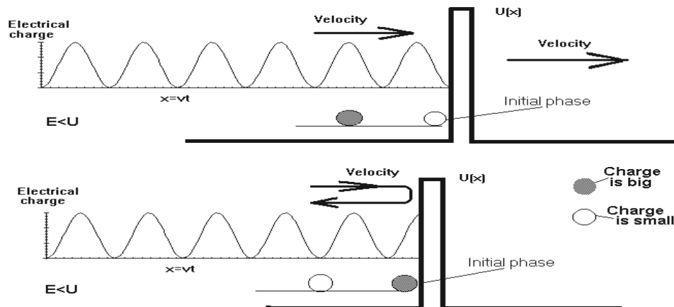
Fig.9. Illustration of the tunnel effect
