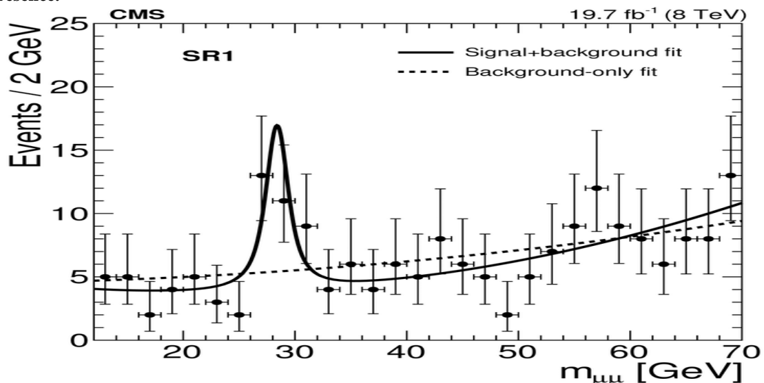
Fig.6. Peak of energy at 28GeV
