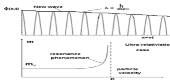
Fig. 3. New wave.
