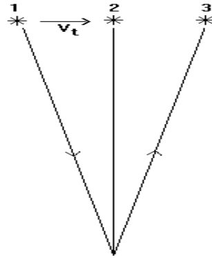
Fig.10. The past (1), verily (2) and the future (3) positions of astronomical object. Portion of light emitted by object in position (1) reaches observer (4) many years after. During this time the object that moves perpendicular to observer with speed v_t , moves to position (2). If at the moment of record portion of light were emitted for point of observation it would meet object in point (3).
