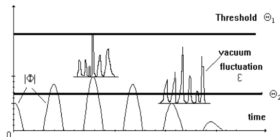
Fig.4. Quantum measurements.
