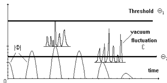
Fig.4. Quantum measurements.
