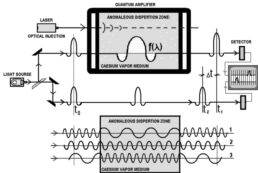
Fig. 5. Experiments of L.Wang - superluminal light propagation.
