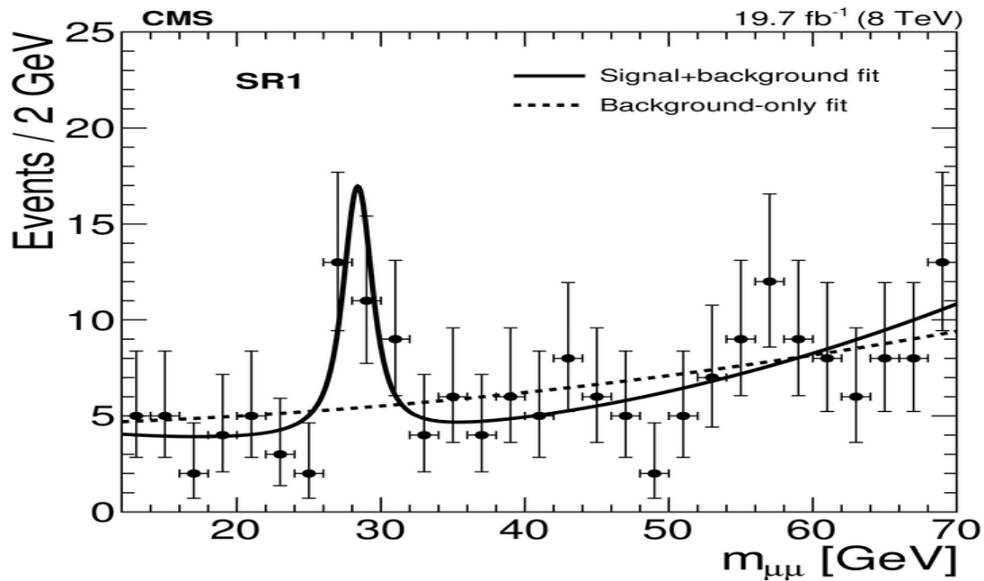
Fig.6. Peak of energy at 28GeV
