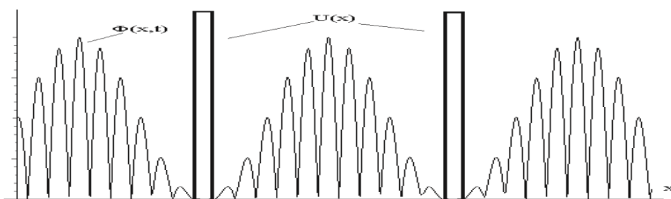
Fig.10. Visual image of particles passing through two potential barriers - scheme of New Maxwell Demon.
